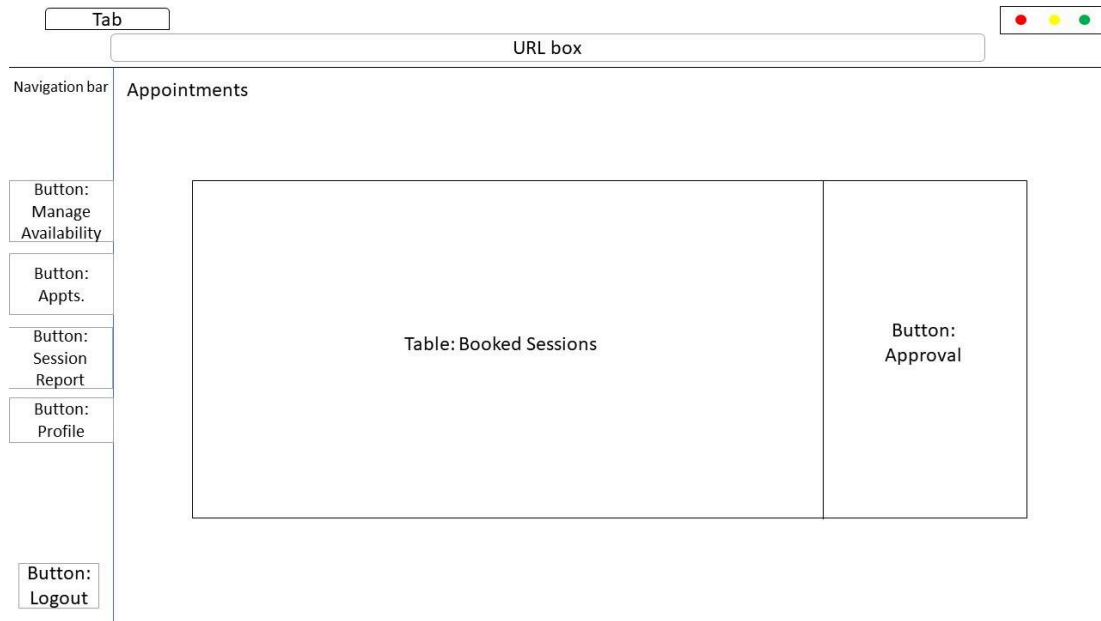
Figure 2.6.10 : Booked Sessions Page
