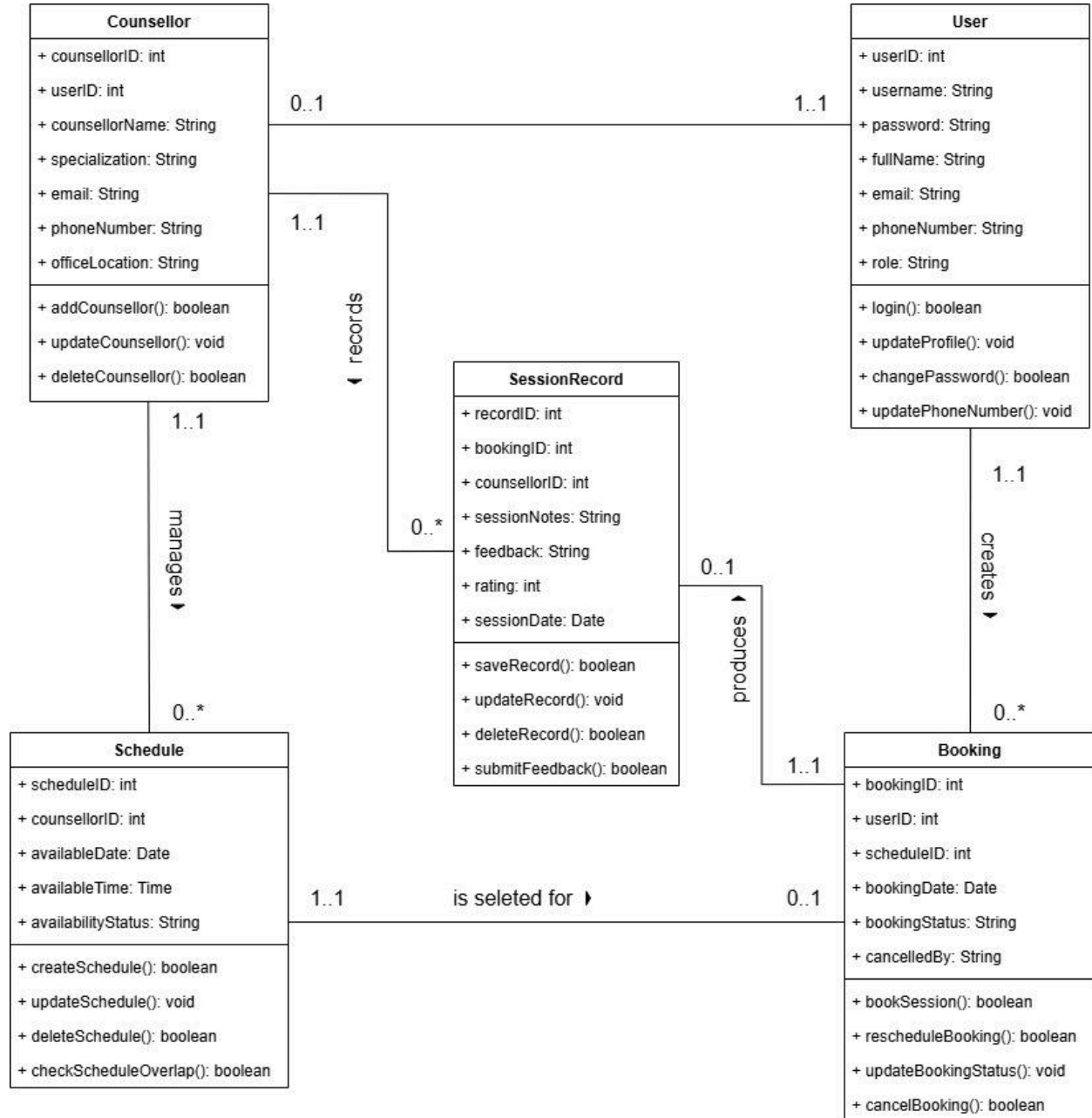
Figure 2.3: Class Diagram of Counseling Session Booking System
