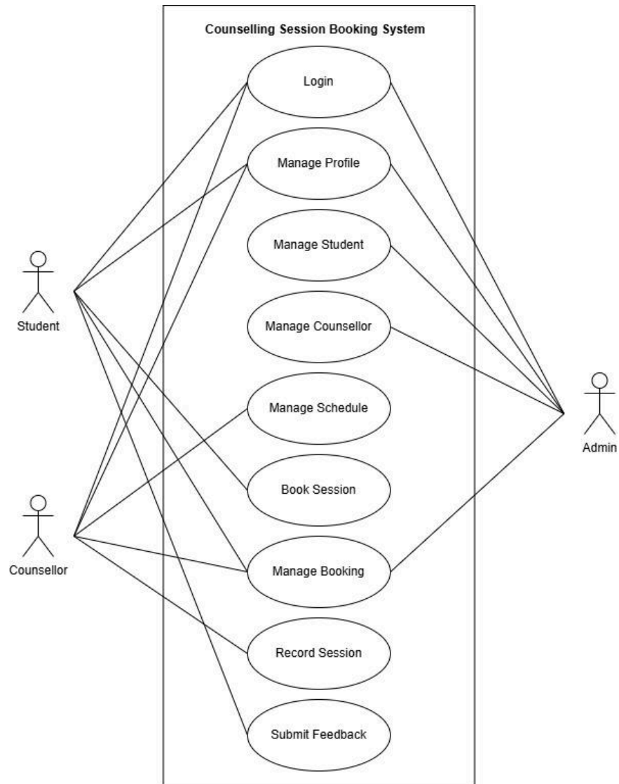
Figure 2.1: Use Case Diagram of Counseling Session Booking System
